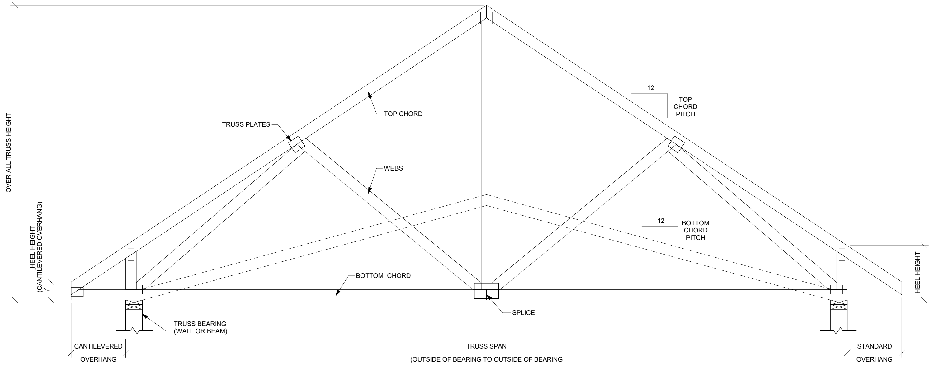
TRUSS INFORMATION DIAGRAM
